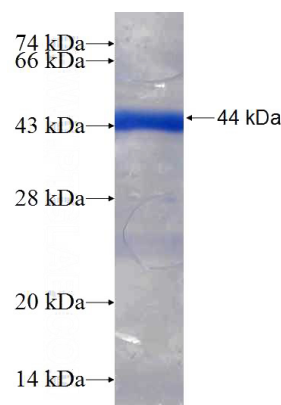
Recombinant Human ADAM7 SDS-PAGE
