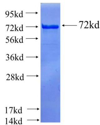
Recombinant human DNMT3A SDS-PAGE
