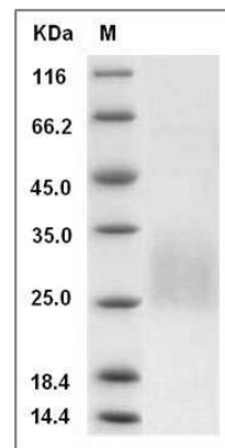
Rat REG4 Protein (His Tag) SDS-PAGE
