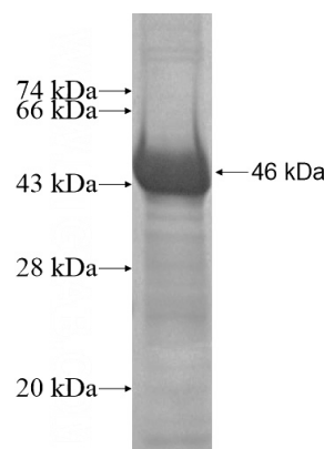
Recombinant Human KCNAB2 SDS-PAGE
