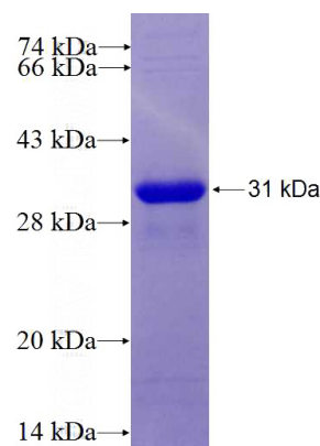
Recombinant Human DAB2 SDS-PAGE
