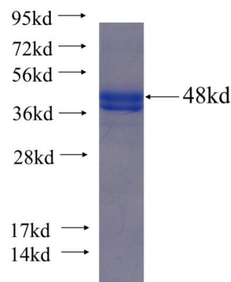
Recombinant Arabidopsis thaliana ARF1A1C SDS-PAGE
