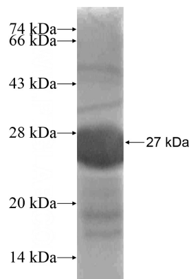
Recombinant Human RHBDL1 SDS-PAGE
