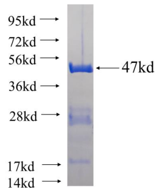
Recombinant human PROX1 SDS-PAGE
