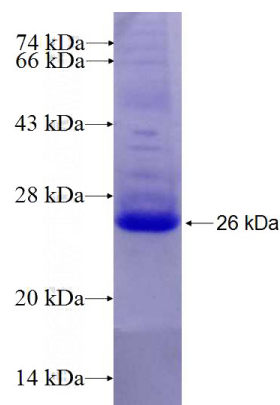
Recombinant Human TRIB1 SDS-PAGE
