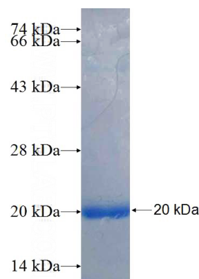
Recombinant Human DOCK4 SDS-PAGE
