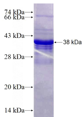
Recombinant Human SLD5 SDS-PAGE
