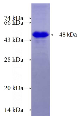
Recombinant Human LUZP4 SDS-PAGE
