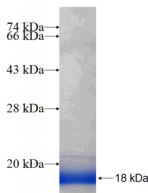
Recombinant Human RBX1 SDS-PAGE
