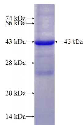
Recombinant Human CYP11B1 SDS-PAGE
