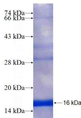
Recombinant Human CH25H SDS-PAGE
