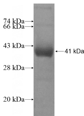
Recombinant Human TBC1D16 SDS-PAGE
