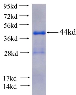
Recombinant human PAICS SDS-PAGE
