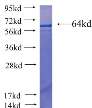
Recombinant human VPS4A SDS-PAGE
