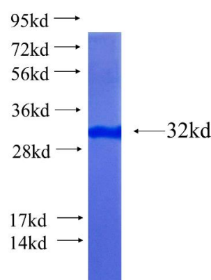
Recombinant human LTBP1 SDS-PAGE
