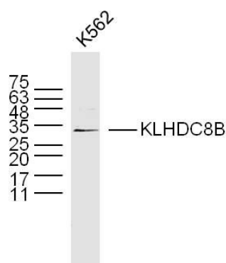
Fig1: Sample:; K562 Cell (Human) Lysate at 30 ug; Primary: Anti- KLHDC8B at 1/300 dilution; Secondary: IRDye800CW Goat Anti-Rabbit IgG at 1/20000 dilution; Predicted band size: 38 kD; Observed band size: 34 kD
