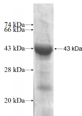
Recombinant Human RNF8 SDS-PAGE
