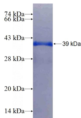
Recombinant Human SLC39A14 SDS-PAGE
