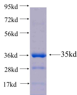
Recombinant human MMS19 SDS-PAGE
