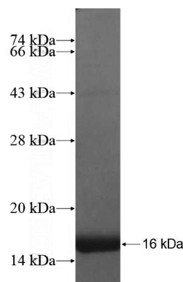
Recombinant Human ADAMTS4 SDS-PAGE
