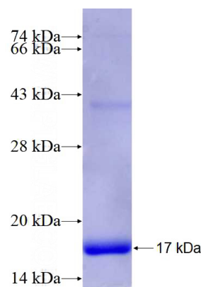
Recombinant Human ITGAV SDS-PAGE
