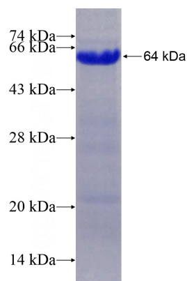
Recombinant Human HRD1 SDS-PAGE
