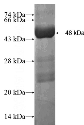
Recombinant Human LAMB4 SDS-PAGE
