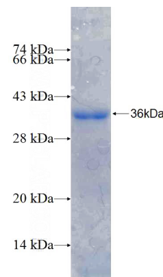
Recombinant Human SNAI2 SDS-PAGE
