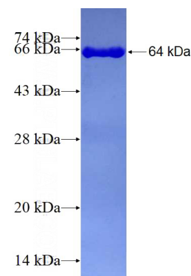
Recombinant Human OAS1 SDS-PAGE
