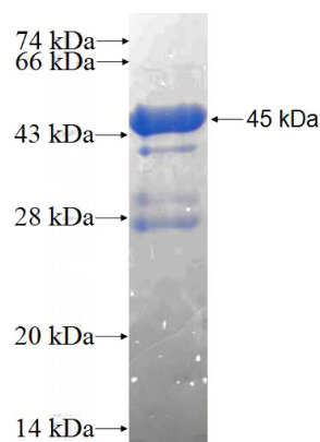
Recombinant Human OCA2 SDS-PAGE
