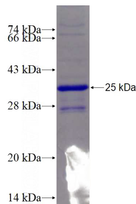
Recombinant Human TEPP SDS-PAGE
