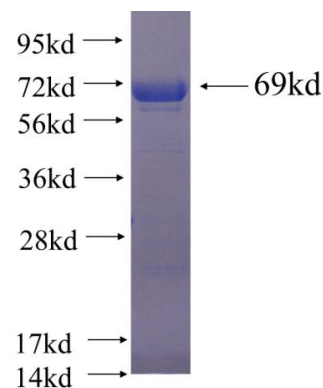
Recombinant human PRKAR1B(Full length) SDS-PAGE
