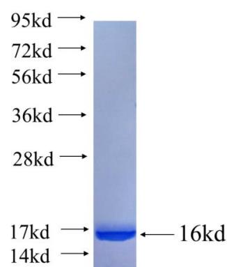
Recombinant human SPRED2 SDS-PAGE
