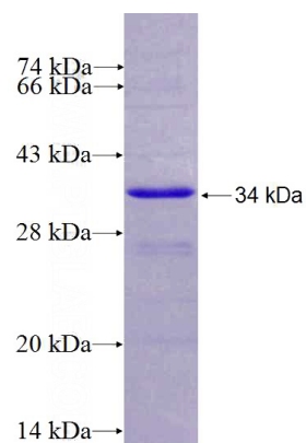
Recombinant Human USP48 SDS-PAGE
