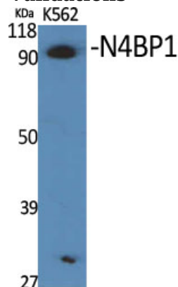
Fig1.; Western Blot analysis of various cells using N4BP1 Polyclonal Antibody cells nucleus extracted by Minute TM Cytoplasmic and Nuclear Fractionation kit (SC-003, Inventibiotech, MN, USA).
