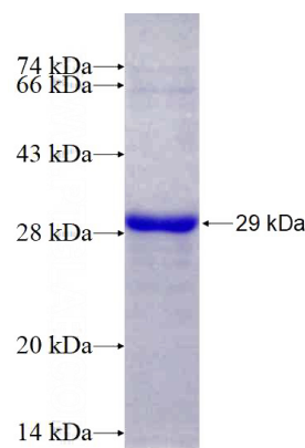
Recombinant Human SPON2 SDS-PAGE
