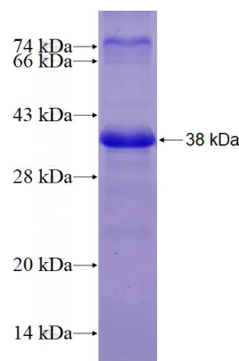
Recombinant Human DTX2 SDS-PAGE
