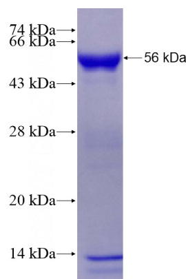
Recombinant Human CCDC83 SDS-PAGE
