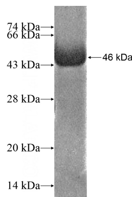
Recombinant Human ASTN1 SDS-PAGE
