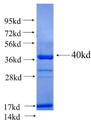
Recombinant human HNF1B SDS-PAGE
