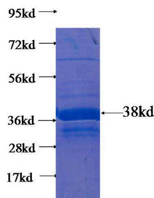
Recombinant human REM2 SDS-PAGE
