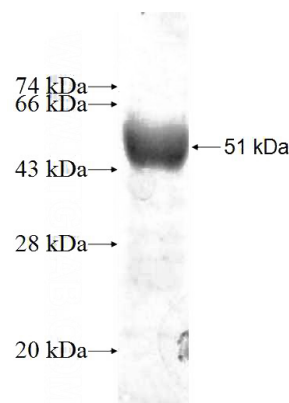
Recombinant Human BHMT SDS-PAGE
