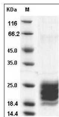
Human IL-9 / Interleukin-9 Protein (His Tag) SDS-PAGE
