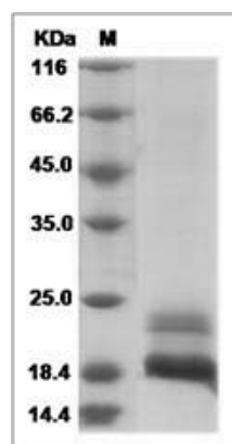
CDNF protein SDS-PAGE
