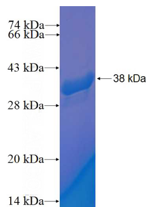
Recombinant Human TCEAL7 SDS-PAGE
