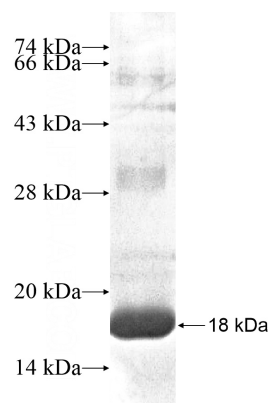
Recombinant Human CNFN SDS-PAGE
