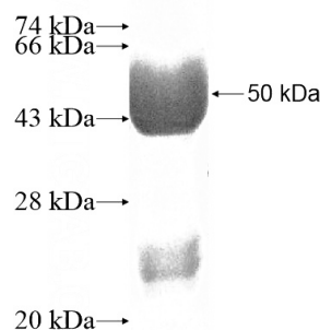
Recombinant Human RAB5B SDS-PAGE
