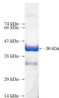
Recombinant Human SH3BGRL3 SDS-PAGE
