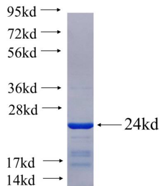
Recombinant human CSN3 SDS-PAGE
