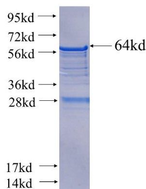
Recombinant human NCRNA00153 SDS-PAGE
